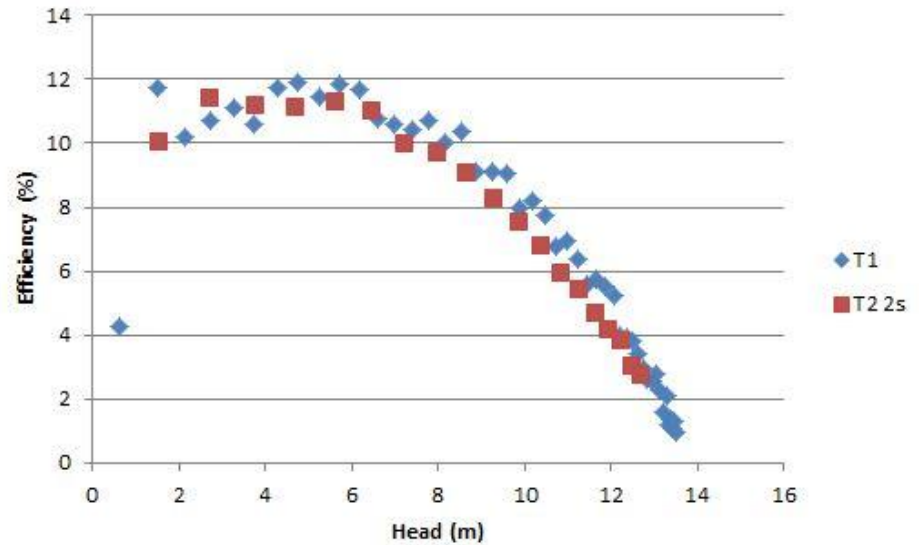
Efficiency graph:
